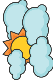
Partly cloudy
